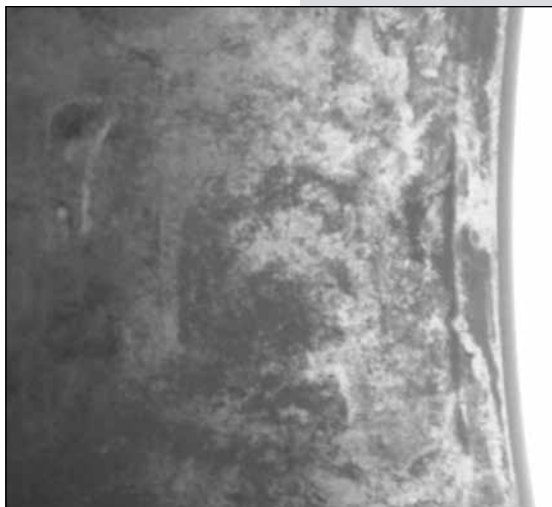
Fig. 47. Classic fretting corrosion from poor fitting practice is depicted here. Relative movement under load between the bearing and its seat caused this worn and corroded condition.
